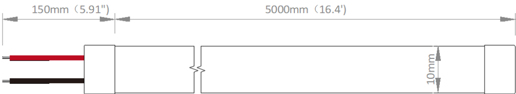
Digital RGB neon light, Top Bending (Vertical Bending)
