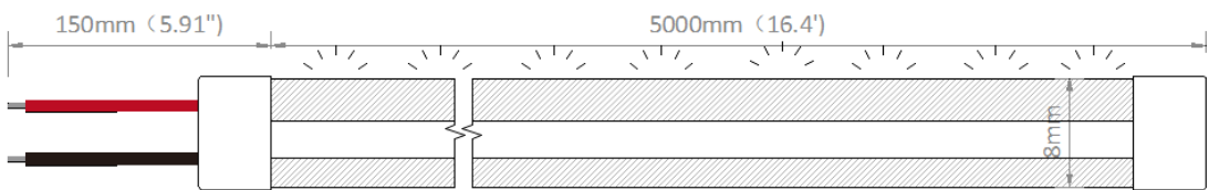
MINI size Neon light, Side Bending (Horizontal Bending)
